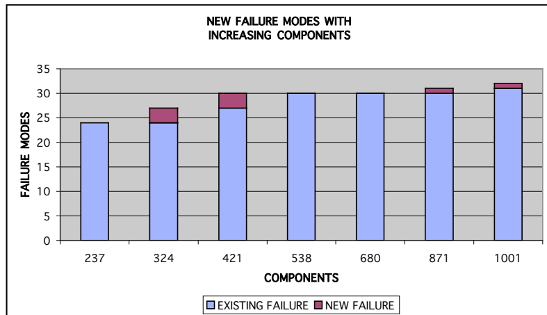
Figure 4. Distinct failure modes with increasing components.
